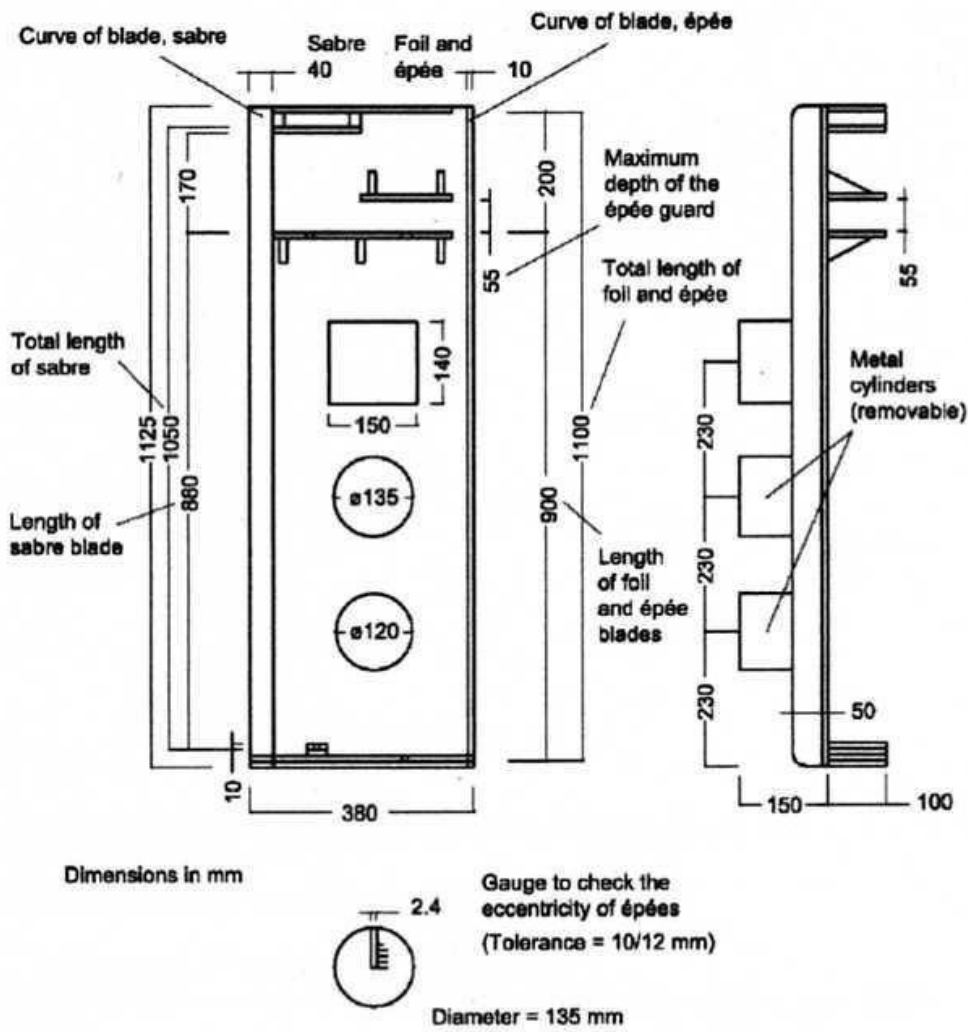
Figure 7. Gauge for checking weapons
